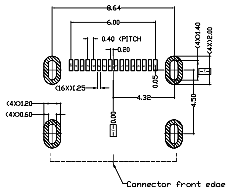
RECOMMENDED P. C. B LAYOUT TOP VIEW TOLERANCES ± 0.05MM
